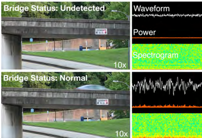
Figure 19: We can monitor bridge structural health using the magnitude and frequency of vibrations as vehicles cross.
